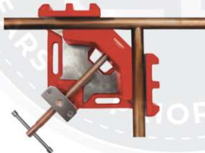
90° Welding Angle Clamp
